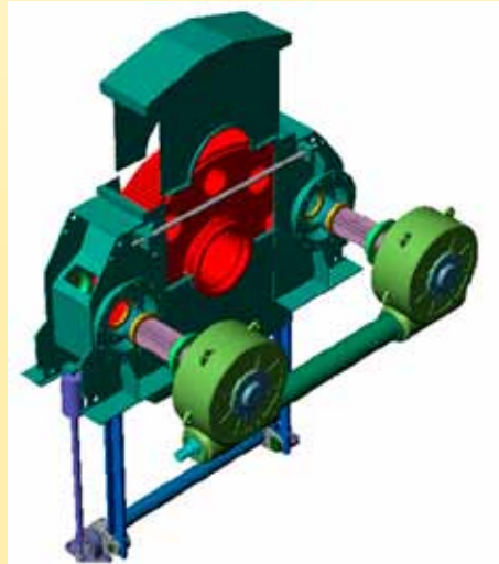
Bogiflex® BFT Horizontal diffuser drive
